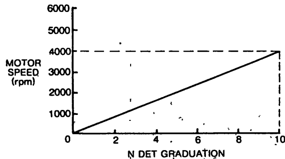
Fig. 8.7 Characteristics of Speed Coincidence Detection Level—Setting
